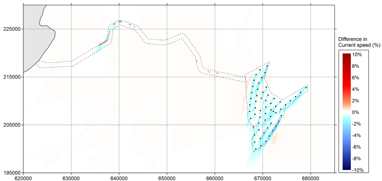
Figure 5.33 Difference in current speed (in percent) between 'Baseline' and 'Option' during neap tide (positive means increase of current speed by option and vice versa) – peak flood
