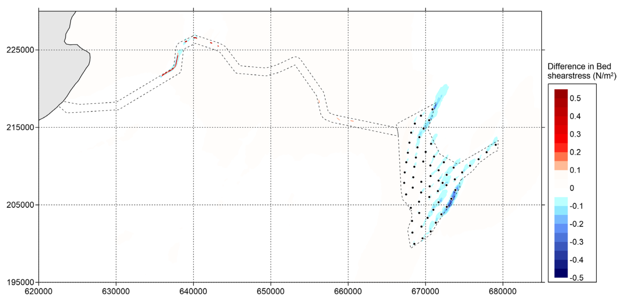
Figure 5.36 Difference in bed shear stress (in \text{N/m}^2 ) between 'Baseline' and 'Option' during spring tide (positive means increase of bed shear stress by option and vice versa) – peak ebb
