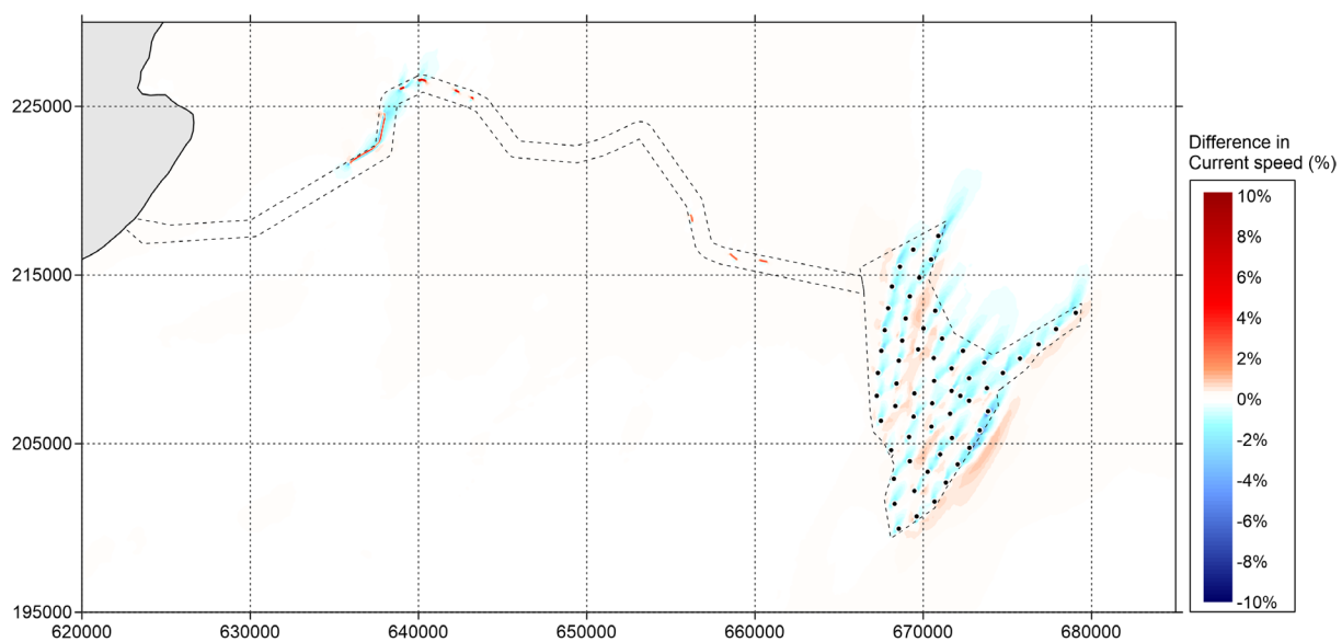
Figure 5.34 Difference in current speed (in percent) between 'Baseline' and 'Option' during neap tide (positive means increase of current speed by option and vice versa) – peak ebb
