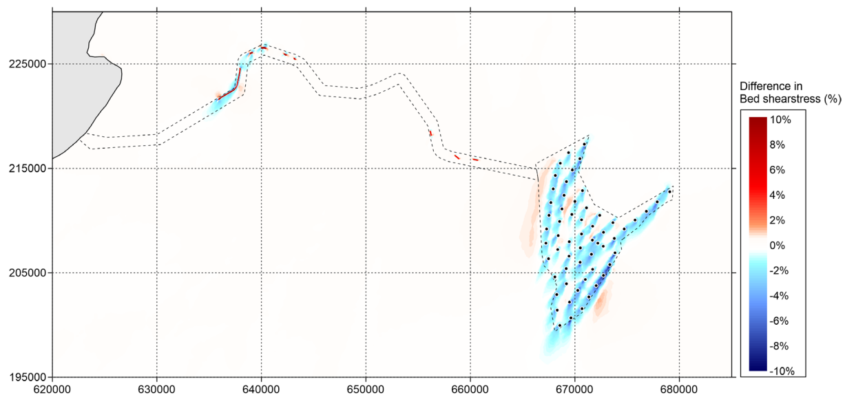
Figure 5.41 Difference in bed shear stress (in percent) between 'Baseline' and 'Option' during neap tide (positive means increase of bed shear stress by option and vice versa) – peak flood
