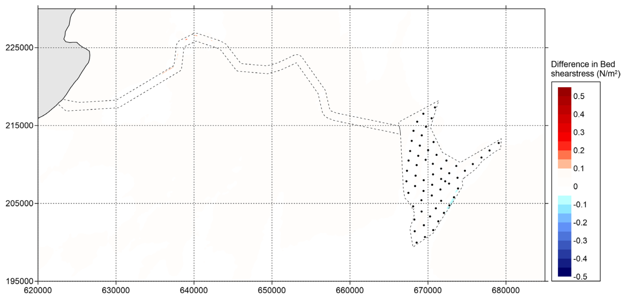
Figure 5.39 Difference in bed shear stress (in \text{N/m}^2 ) between 'Baseline' and 'Option' during neap tide (positive means increase of bed shear stress by option and vice versa) – peak flood
