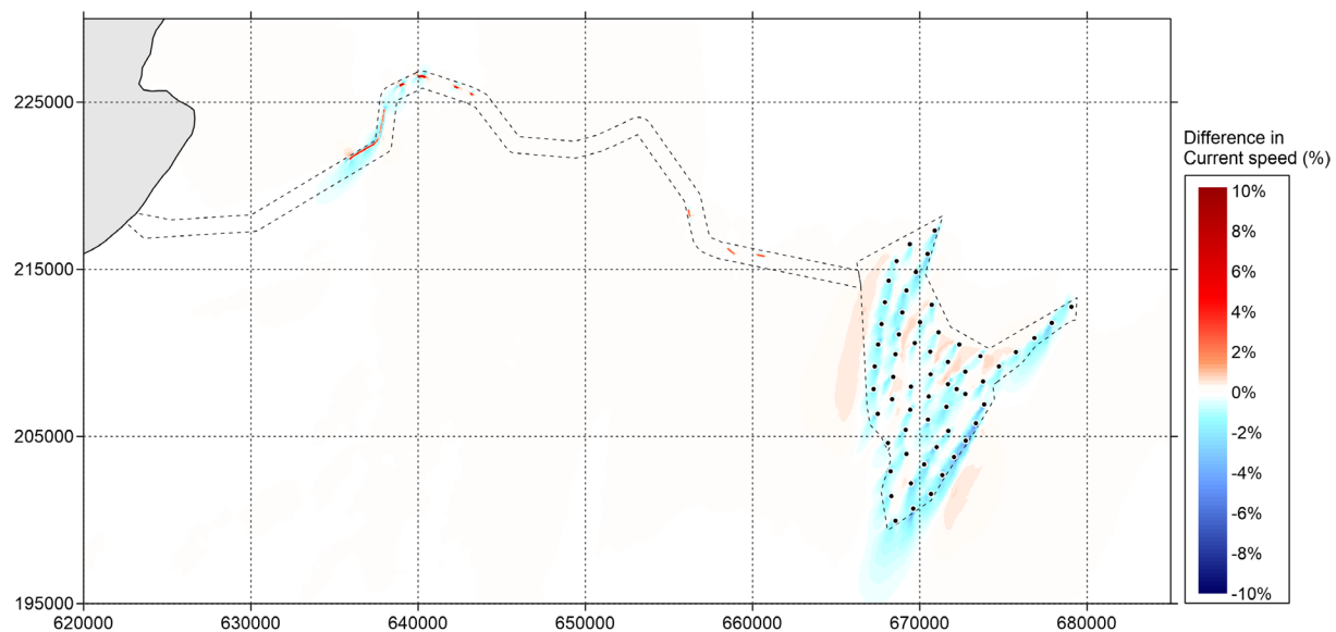
Figure 5.29 Difference in current speed (in percent) between 'Baseline' and 'Option' during spring tide (positive means increase of current speed by option and vice versa) – peak flood
