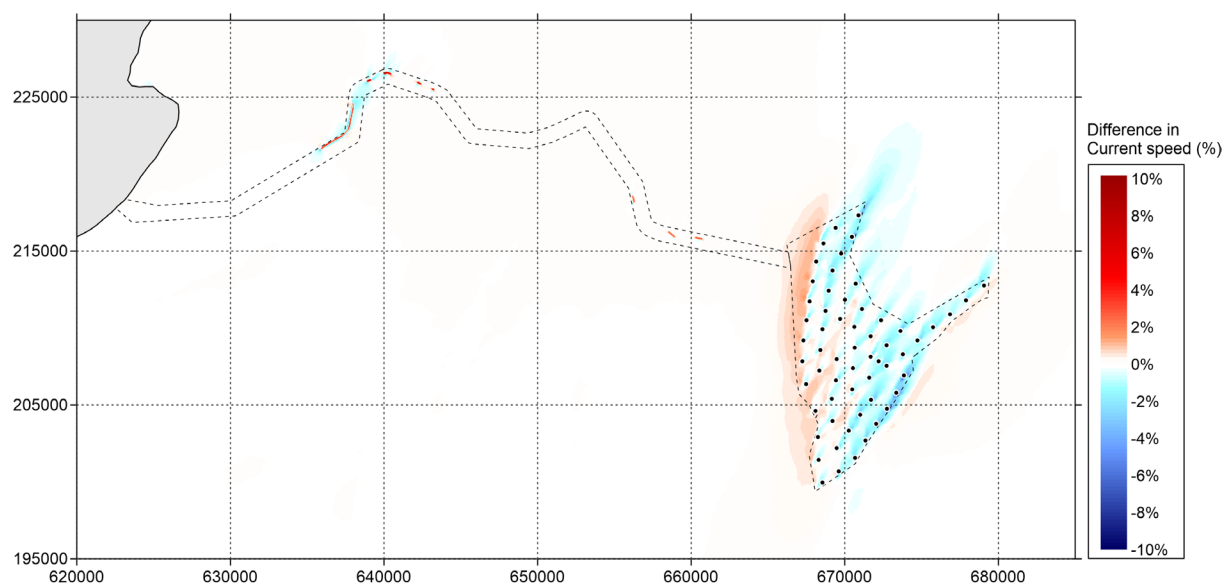
Figure 5.30 Difference in current speed (in percent) between 'Baseline' and 'Option' during spring tide (positive means increase of current speed by option and vice versa) – peak ebb
