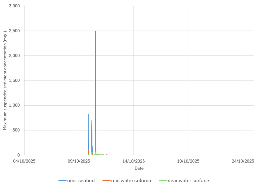
Figure 7.40 Time series of suspended sediment concentration at P1 during seabed preparation for array structures (larger WTGs) near seabed, middle of water column and near water surface
