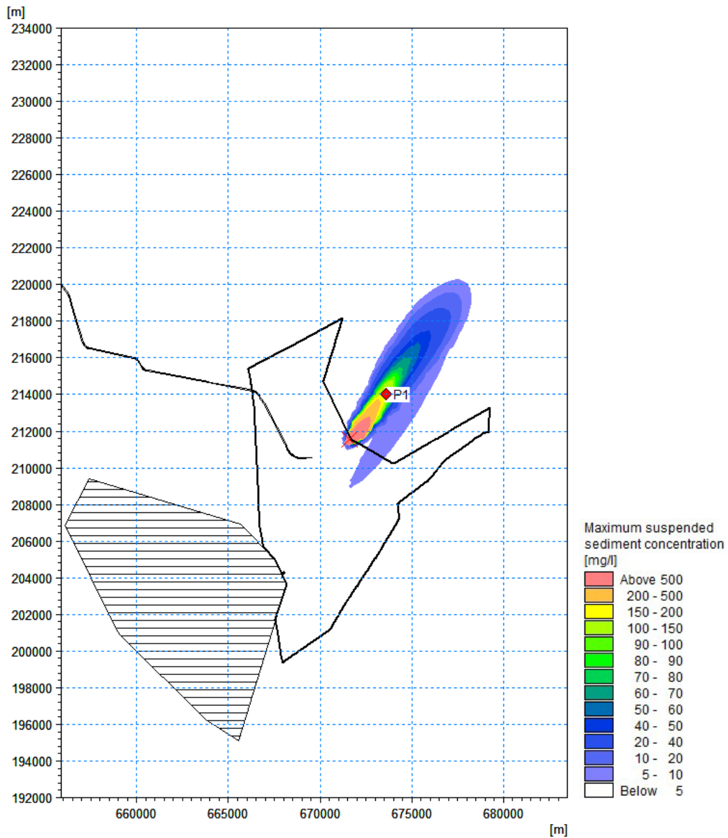
Figure 7.97 Maximum suspended sediment concentration during array disposal occurring near the water surface – Peak ebb during spring tide ('Sandwaves' material)
