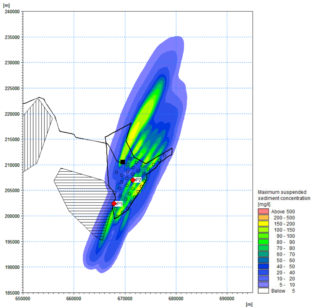
Figure 7.33 Maximum suspended sediment concentration during seabed preparation operations for smaller WTGs layout structures occurring near the water surface (red points = time series extraction points, vertical hashed area = MLS SAC, horizontal hashed area = KKE MCZ)
