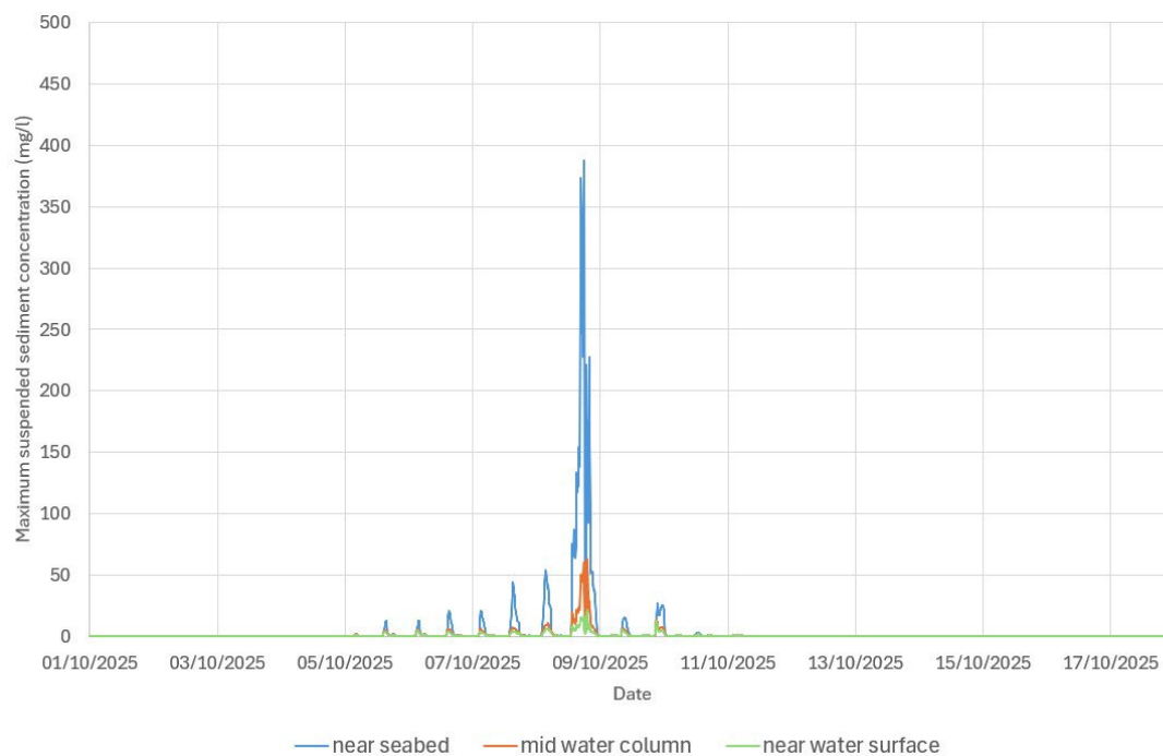
Figure 7.10 Time series of suspended sediment concentration at P1 during offshore export cable trenching near seabed, middle of water column and near water surface (inside SAC)
