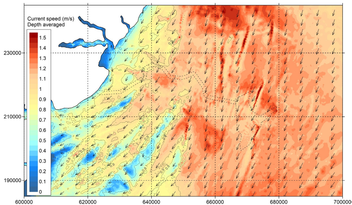
Figure 5.19 Baseline - Current speed during spring tide - peak flood
