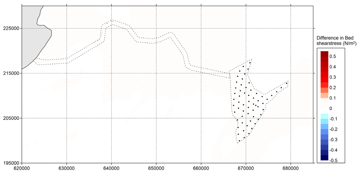
Figure 5.40 Difference in bed shear stress (in \text{N/m}^2 ) between 'Baseline' and 'Option' during neap tide (positive means increase of bed shear stress by option and vice versa) – peak ebb
