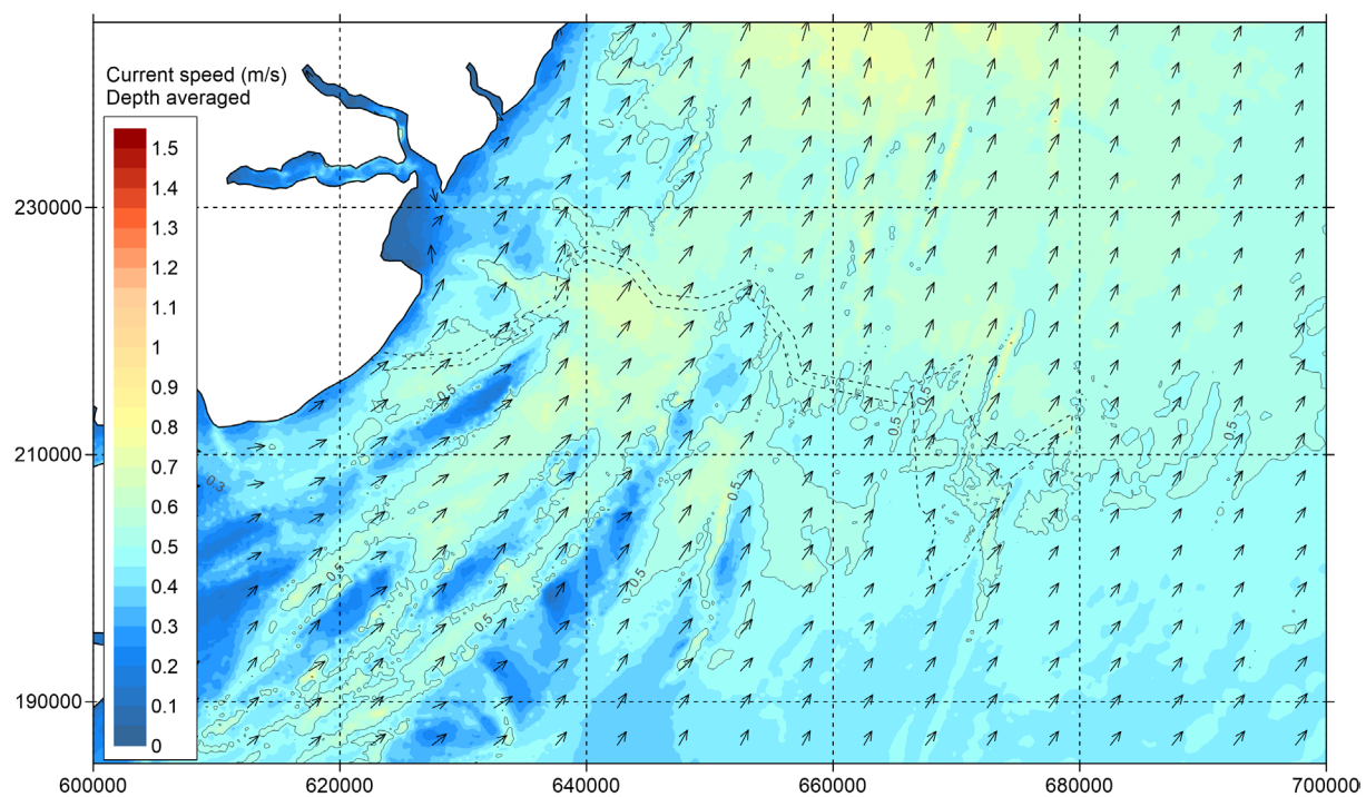
Figure 5.22 Baseline - Current speed during neap tide - peak ebb
