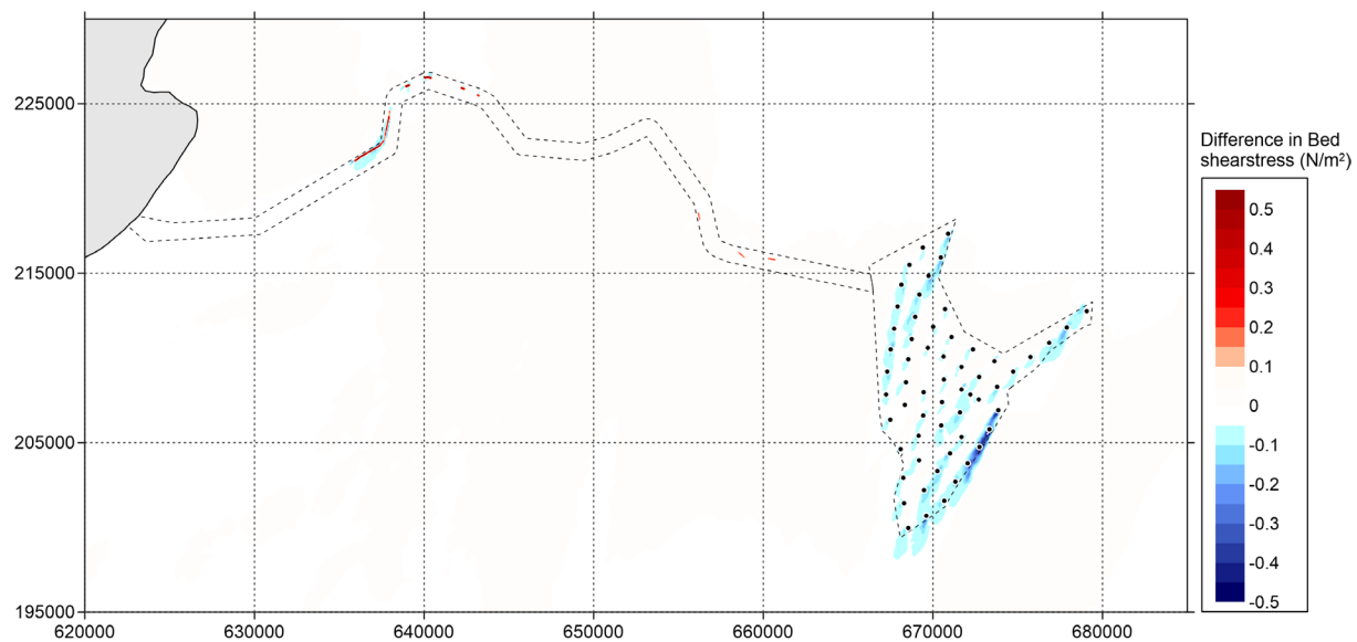
Figure 5.35 Difference in bed shear stress (in \text{N/m}^2 ) between 'Baseline' and 'Option' during spring tide (positive means increase of bed shear stress by option and vice versa) – peak flood
