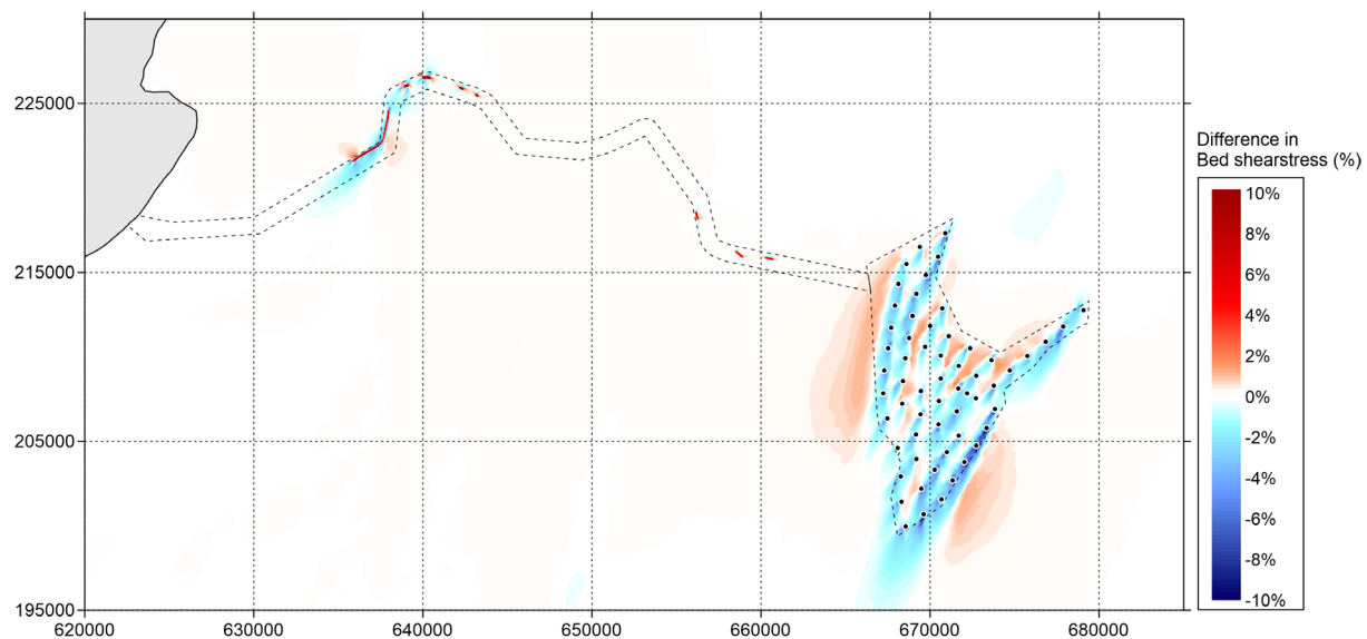
Figure 5.37 Difference in bed shear stress (in percent) between 'Baseline' and 'Option' during spring tide (positive means increase of bed shear stress by option and vice versa) – peak flood
