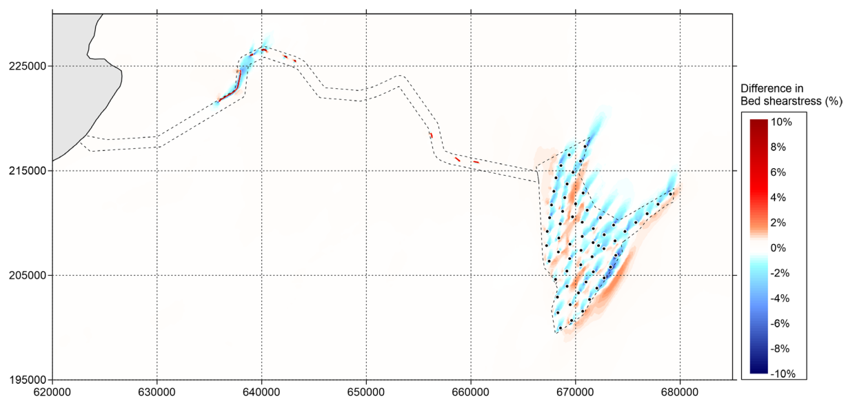
Figure 5.42 Difference in bed shear stress (in percent) between 'Baseline' and 'Option' during neap tide (positive means increase of bed shear stress by option and vice versa) – peak ebb
