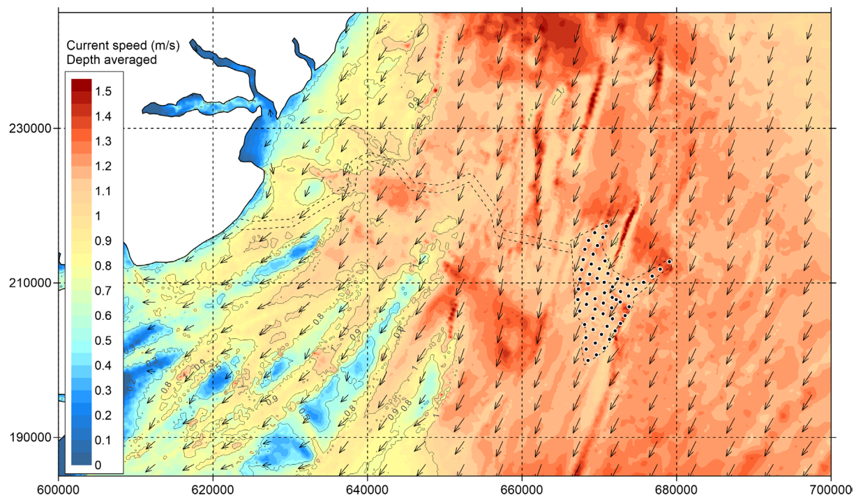
Figure 5.23 Option - Current speed during spring tide - peak flood
