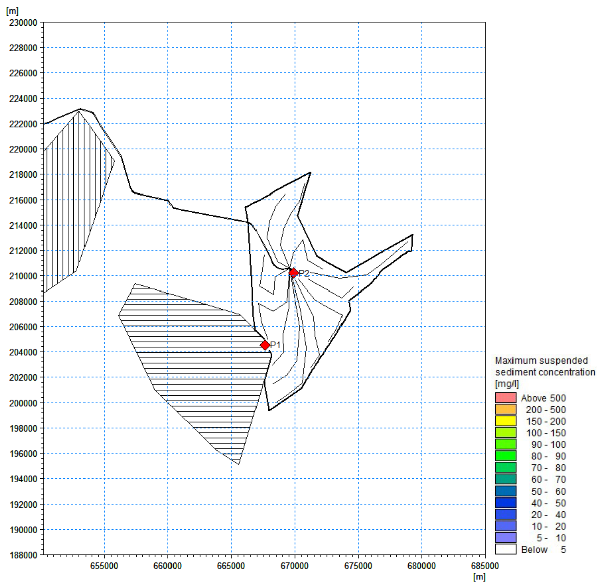
Figure 7.51 Maximum suspended sediment concentration during array cable trenching operations occurring near the water surface
