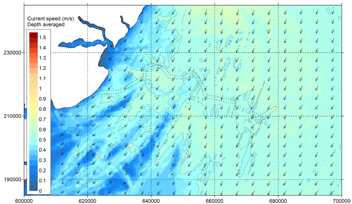
Figure 5.21 Baseline - Current speed during neap tide - peak flood
