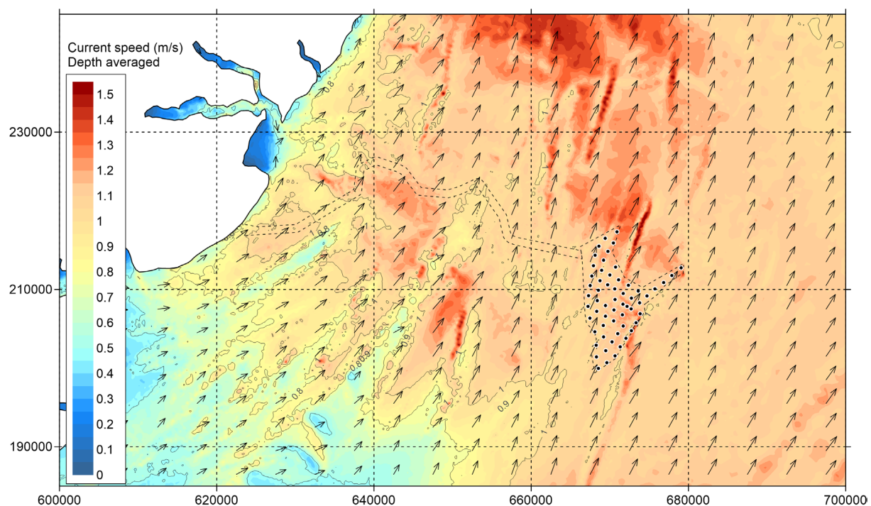
Figure 5.24 Option - Current speed during spring tide - peak ebb
