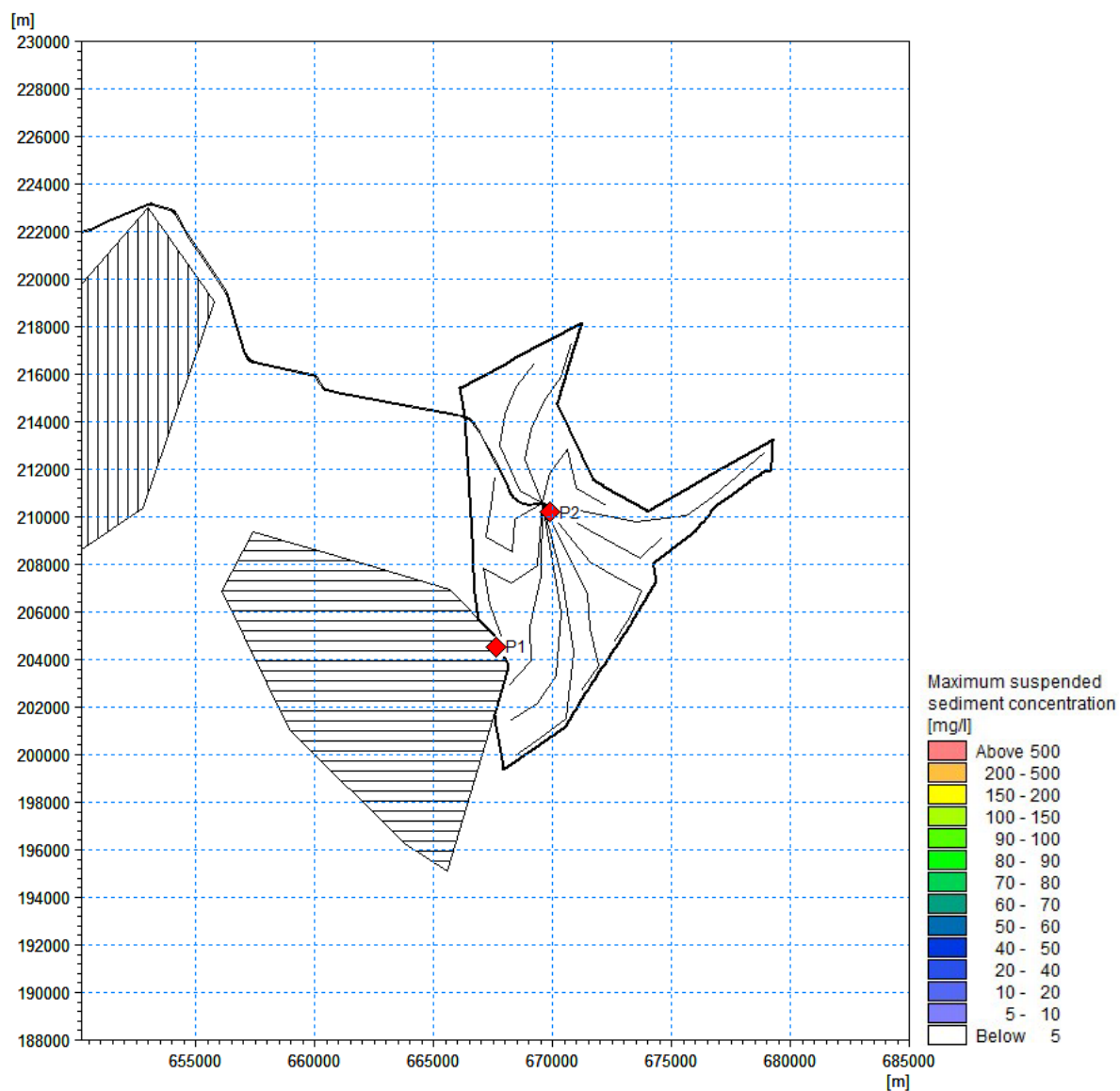
Figure 7.50 Maximum suspended sediment concentration during array cable trenching operations occurring in the middle of water column (red points = time series extraction points vertical hashed area = MLS SAC, horizontal hashed area = KKE MCZ)
