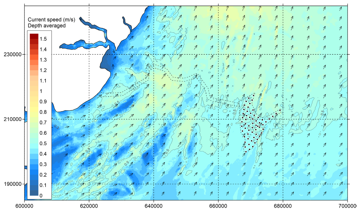
Figure 5.26 Option - Current speed during neap tide - peak ebb
