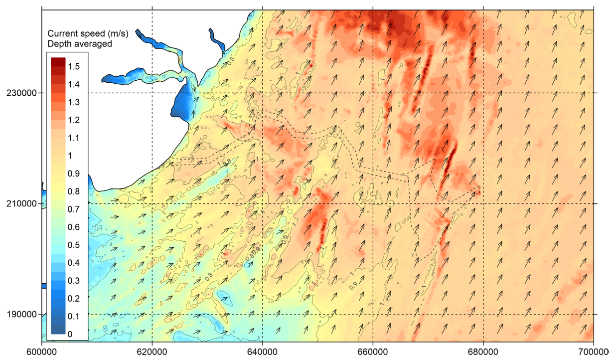
Figure 5.20 Baseline - Current speed during spring tide - peak ebb
