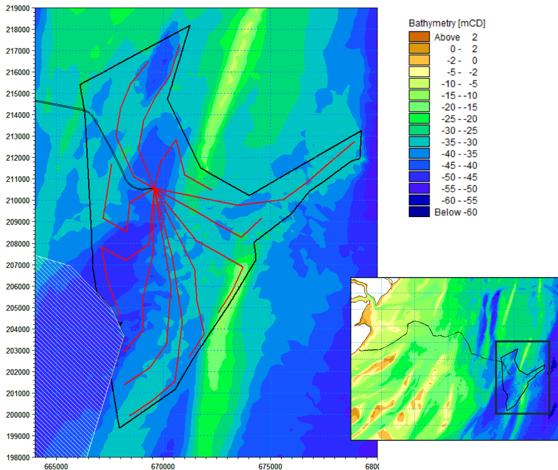
Figure 6.11 Location of array cable trenching activity (red line) white hatch = MCZ
