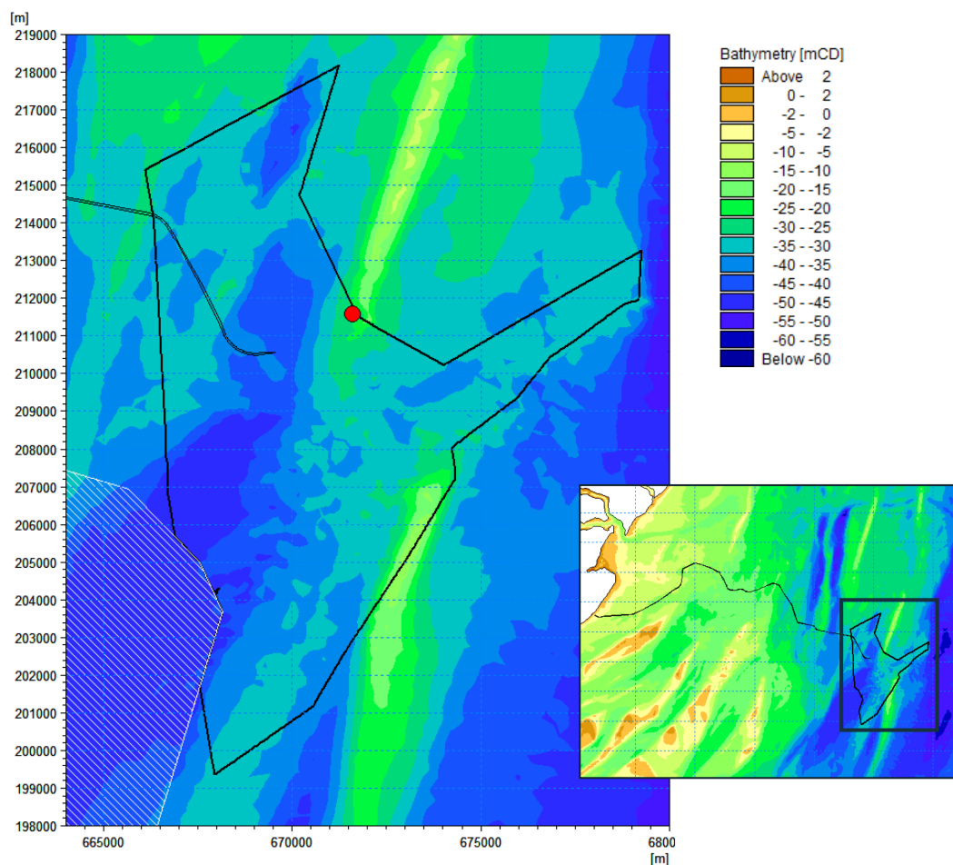
Figure 6.12 Location of sediment disposal (white hatched area = KKE MCZ)
