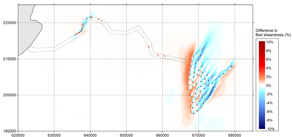
Figure 5.38 Difference in bed shear stress (in percent) between 'Baseline' and 'Option' during spring tide (positive means increase of bed shear stress by option and vice versa) – peak ebb
